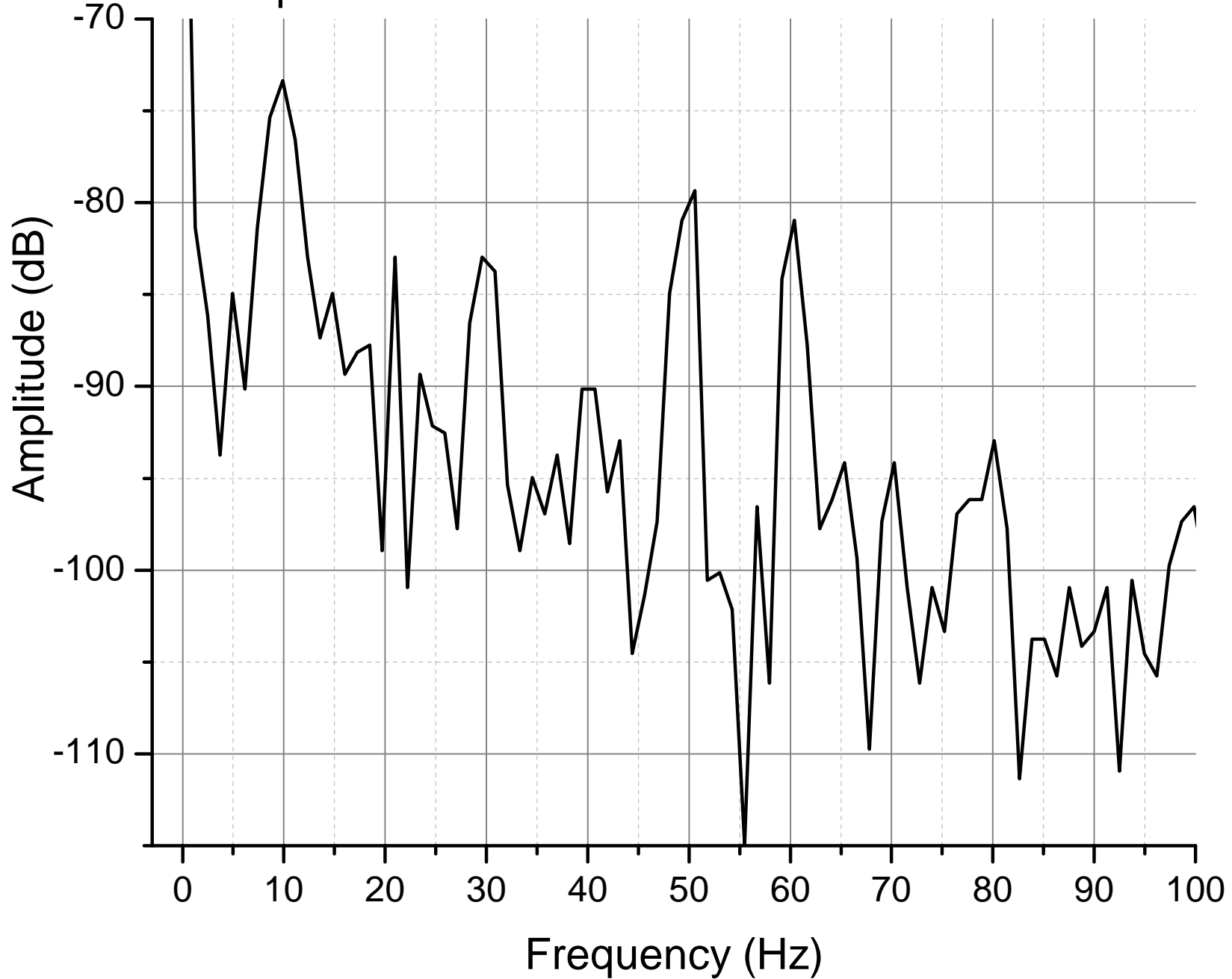
Geophone 20DX - 10 - 395
